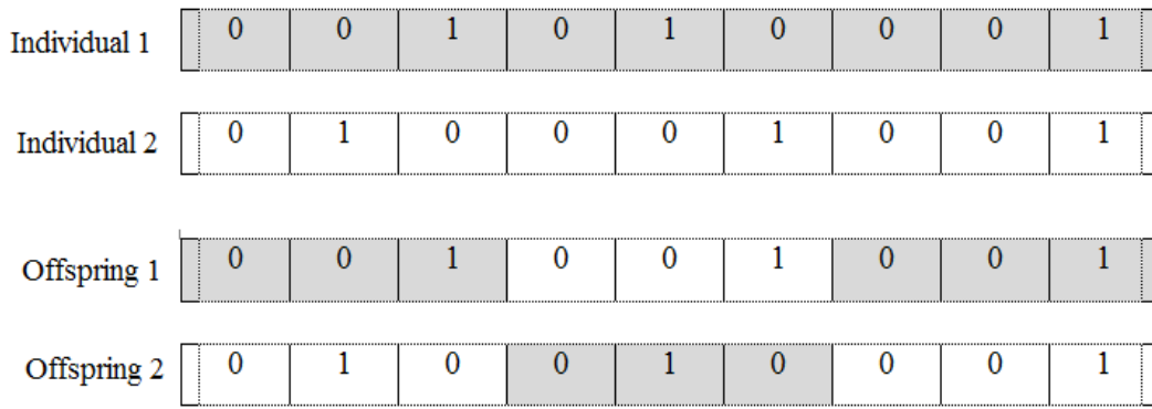
Figure 3: Two-Point Crossover
