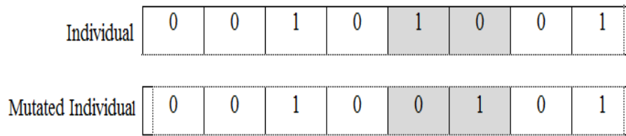
Figure 4: Mutation Procedure
